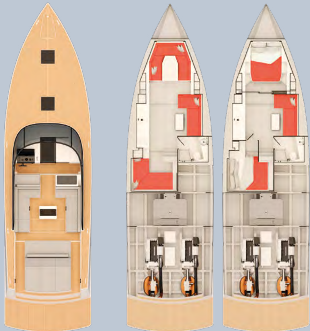
Top View
